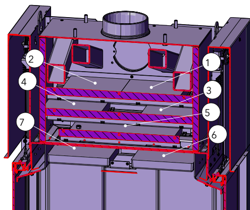
Abb. 20: 75x35x45 S3 2.0
