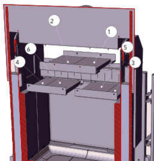
Abb. 24: 80x64 S/SII
